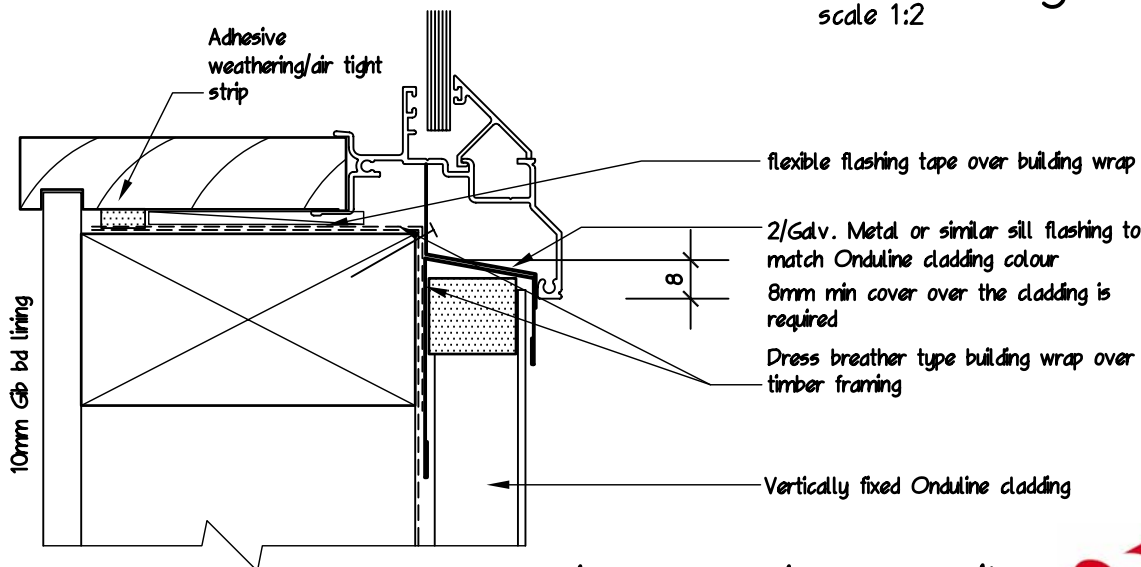
Window sill detail scale 1:2
