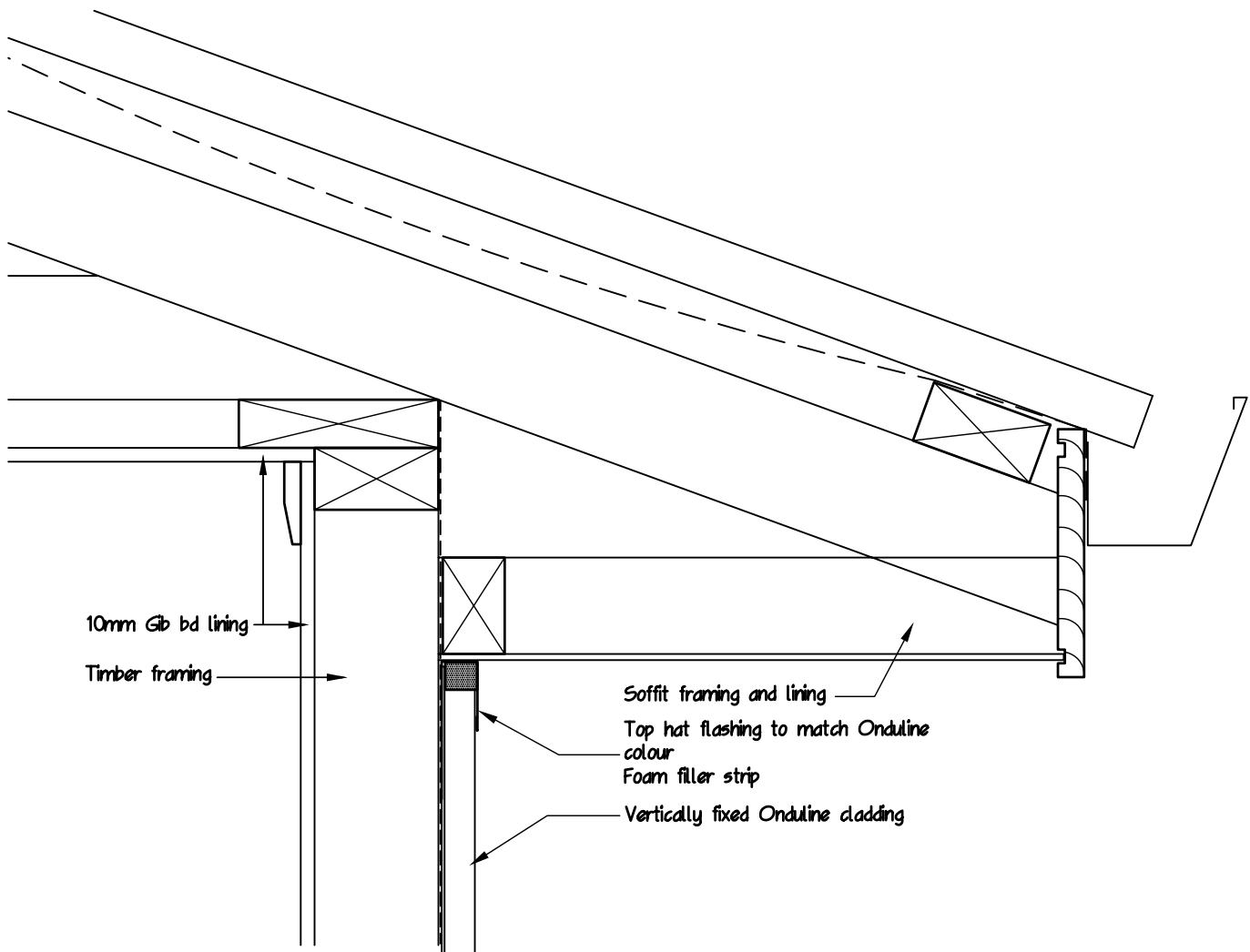
Eaves detail scale 1:5
