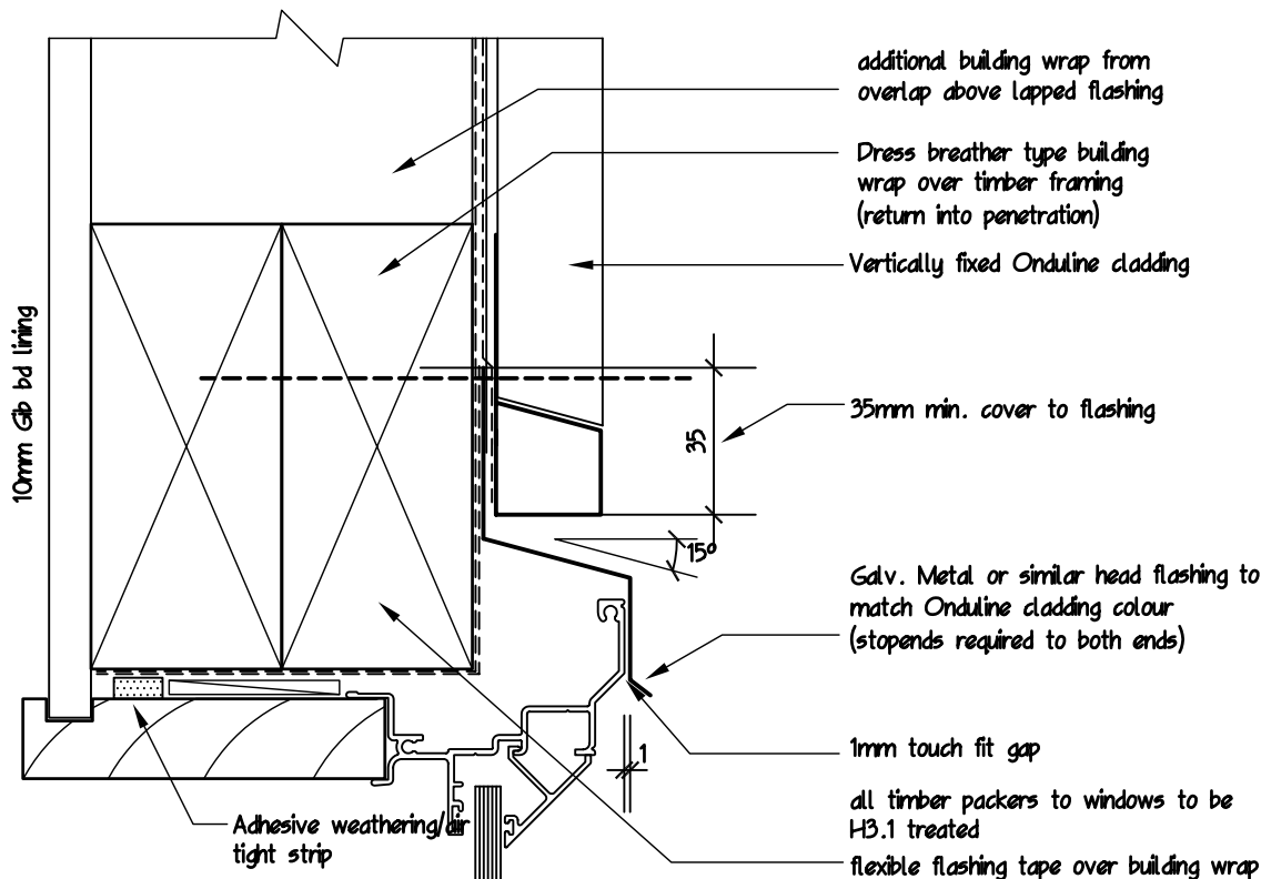
Window head detail scale 1:2
