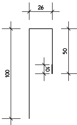
Flashing detail scale 1:2
